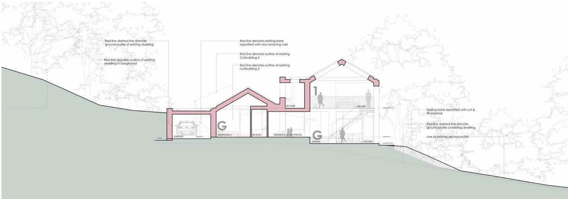
Illustrative Building Section - Proposed Dwelling
