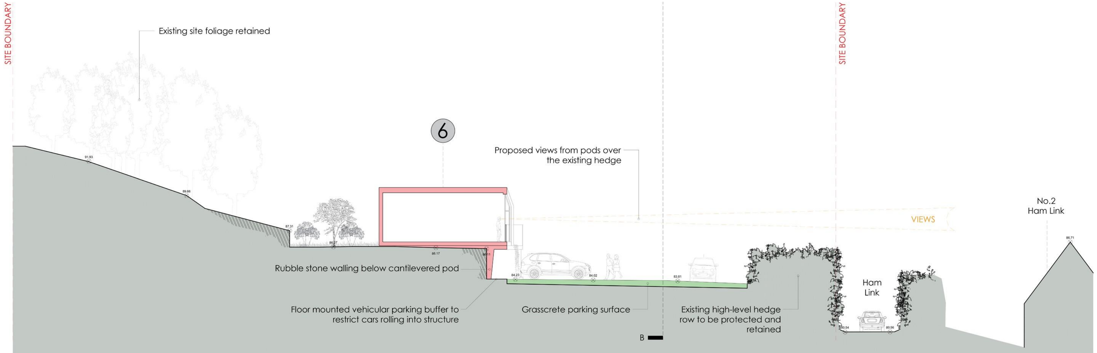
Illustrative site section
